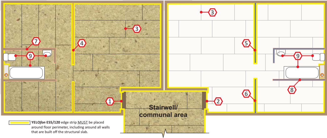
1 Door threshold - Chipboard + Plasterboard plank
