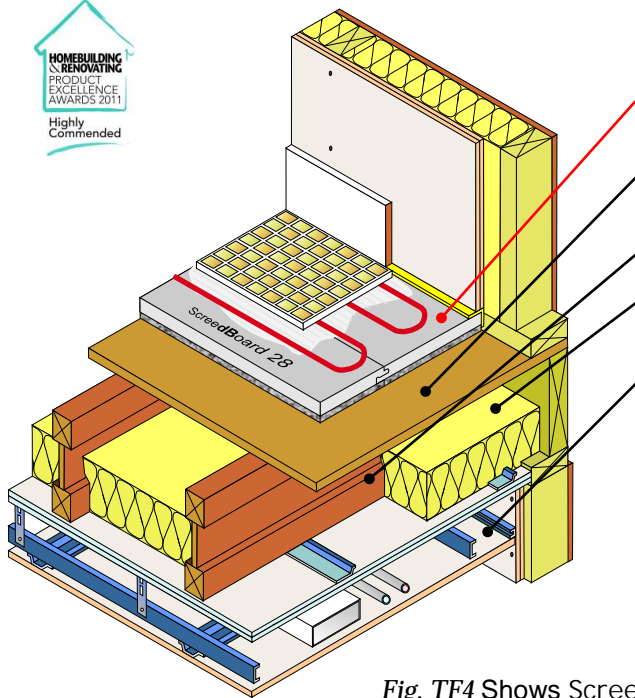
Fig. TF4 Shows ScreedBoard® 28 with optional electric underfloor heating
